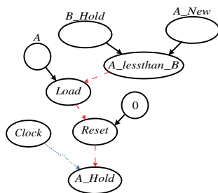
Fig. 4. Relation tree of A\_Hold hand side of assignments and are connected using data arcs.
