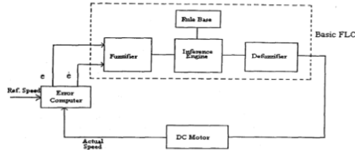
Fig.3 basic function of fuzzy logic controller
