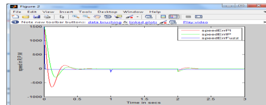
Fig 13. Comparative Speed Error Scope
