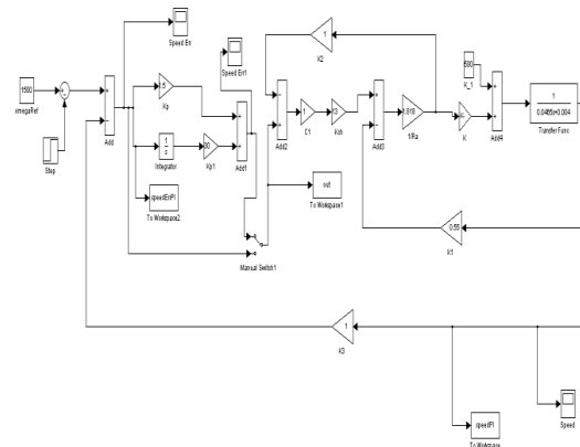
Fig 6. Basic model of P-I controller
