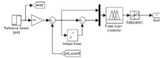
Fig 10. Block Diagram of FLC
