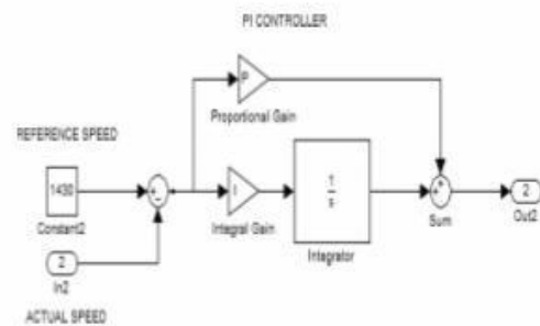
Fig 6. Basic model of P-I controller
