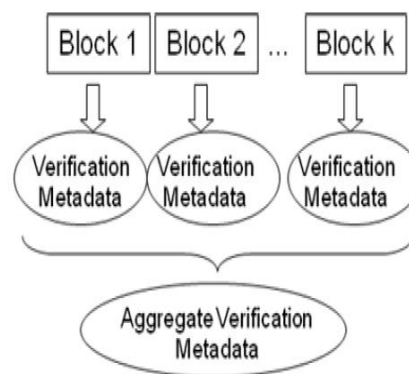
—Fig1 Homomorphic authenticator
