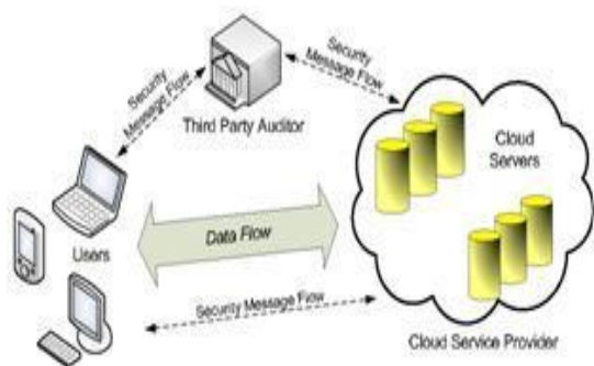
—Fig The architecture of cloud data storage service
