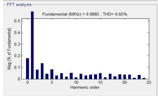
Fig.13.Total harmonic distortion of load voltage with DPFC
