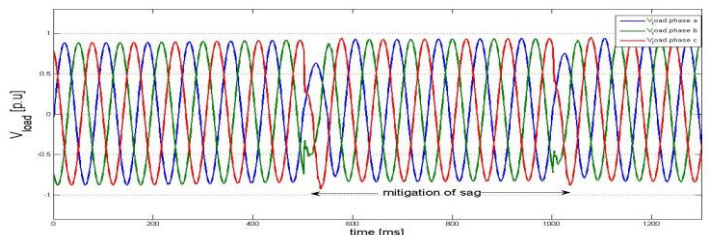
Fig.9. Mitigation of three-phase load voltage sag with DPFC
