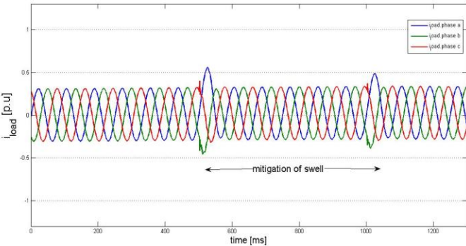
Fig.11.Mitigation of three-phase load current swell with DPFC
