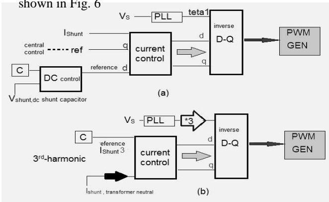
Fig.6. The shunt control configuration: (a) for fundamental frequency (b) for third-harmonic frequency
