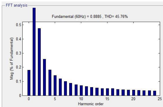
Fig.12.Total harmonic distortion of load voltage without DPFC
