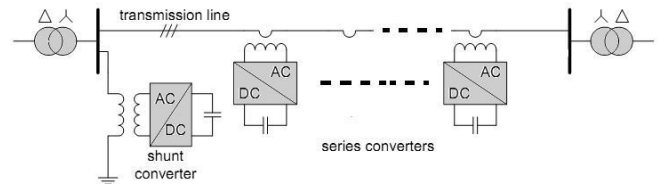
Fig.1.The DPFC Structure
