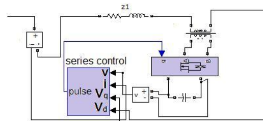
Fig.4.Block diagram of the series converters in Matlab/Simulink.
