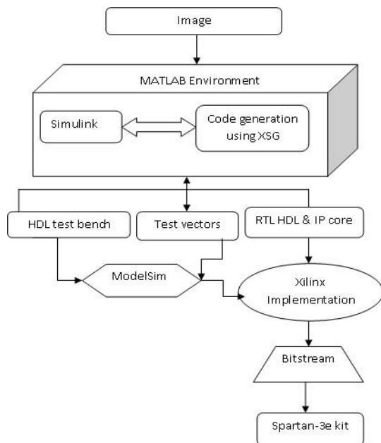
Fig-1 Design flow
