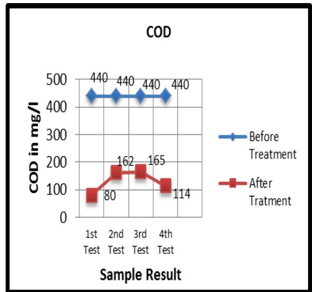
Fig.3.COD value before and after
