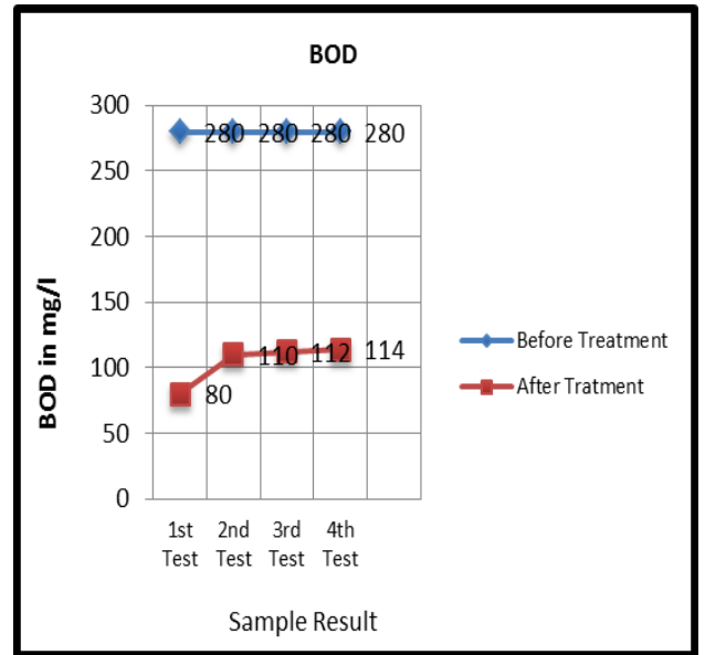
Figure 5.3 BOD value before and after.
