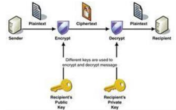
Figure 3: Asymmetric Key Cryptography.
