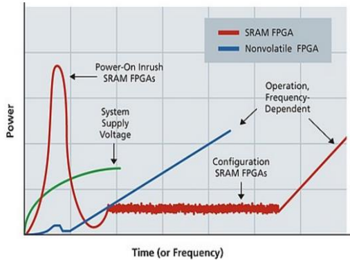
Fig 1: Volatile SRAM FPGA vs. Nonvolatile True Flash FPGA Current
