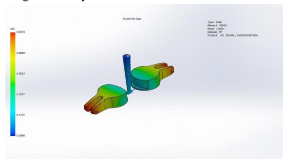
Figure 5. Filling of material in upper part of component
