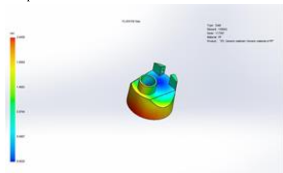
Figure 6. Filling of material in lower part of component
