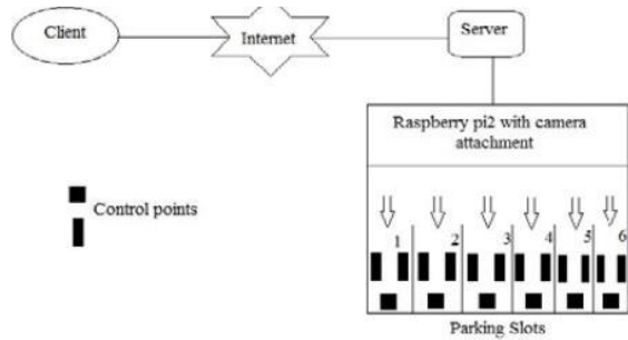
Fig.2. Structure of Smart Parking System
