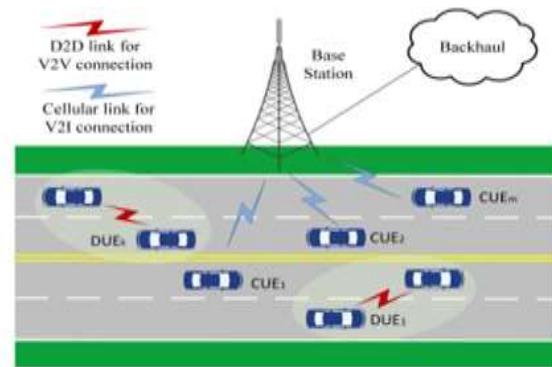
Fig. 1. D2D-enabled vehicular communications for both V2I and V2V links. In this paper, we propose to support both types of vehicular connections, i.e., V2I and V2V links, under the D2D-enabled cellular architecture where the V2I connectivity is enabled by macro cellular link and the V2V connectivity is supported through localized D2D link to achieve the dual benefits of D2D-enabled cellular networks. We base resource management on slow fading parameters and statistical information of the channel instead of instantaneous CSI to address the challenges caused by the inability to track fast changing wireless channels. Moreover, we identify and incorporate into problem formulation differentiated QoS requirements for V2I and V2V links in correspondence with their supported applications. That is, high link capacity is desired for V2I connections while safety-critical information of V2V connections places greater emphasis on link reliability. Sum and minimum ergodic capacities (long-term average over fast fading) of V2I links are maximized with a minimum QoS guarantee for V2I and V2V links, where the V2V link reliability is ensured by maintaining the outage probability of received SINR below a small threshold. To the best of our knowledge, this is the first work that jointly
