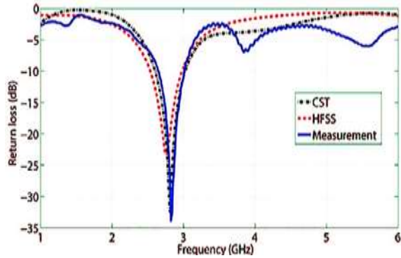
Fig.4. results of frequency and return in loss (Dbi)
