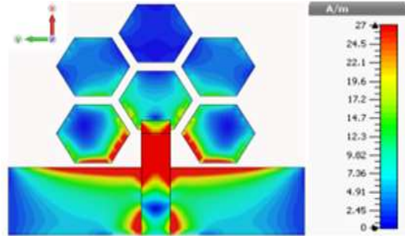
Fig.6. surface current distribution at 32 GHz
