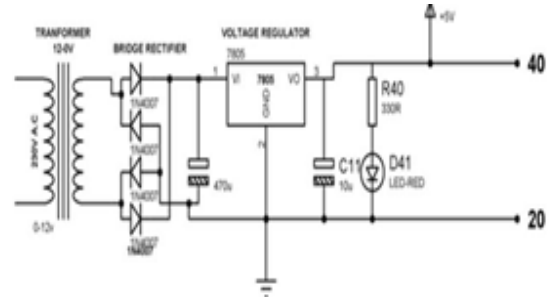
Fig -2: Power Supply Diagram
