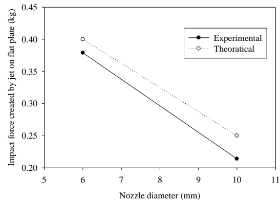
Fig. 3. Comparison between theoretical and experimental impact created by water jet on flat vane
