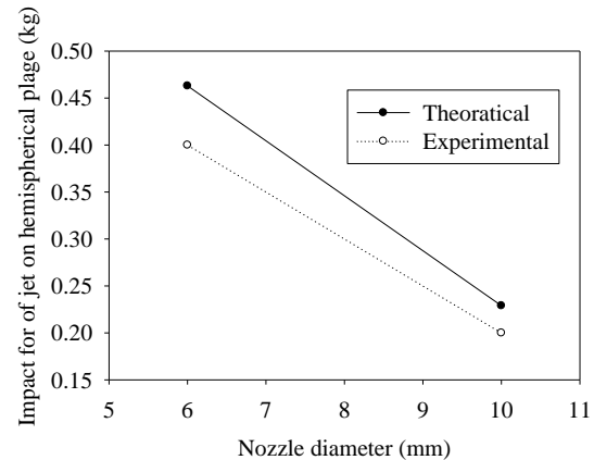
Fig. 4. Comparison between theoretical and experimental impact created by water jet on hemispherical vane
