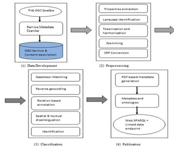
Figure 4: Linked Data Model Process
