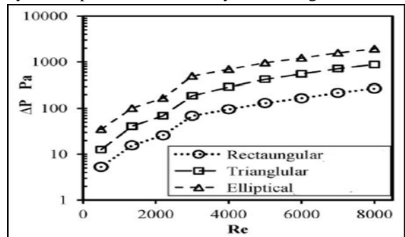
Fig. 3. Variation in pressure drops with Reynolds number
