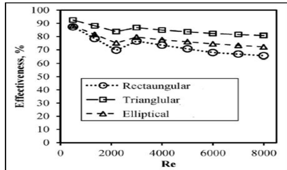
Fig. 2. Variation in effectiveness with Reynolds number
