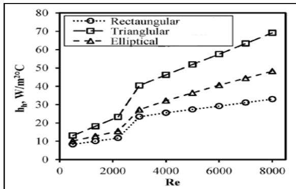
Fig. 4. Variation in HTC with Reynolds number
