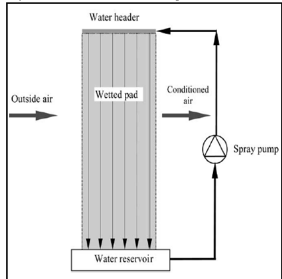
Fig. 3. Working of evaporative cooler
