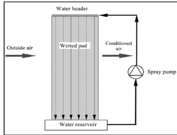
Fig. 3. Working of evaporative water cooler
