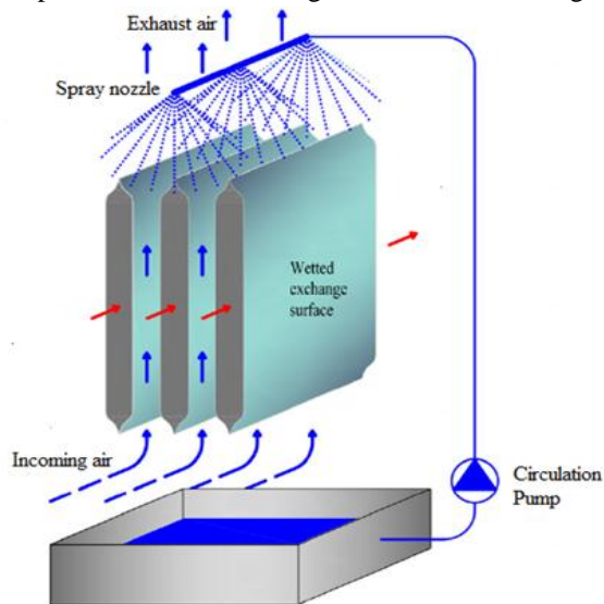
Fig. 1. Evaporation principle in water cooling
