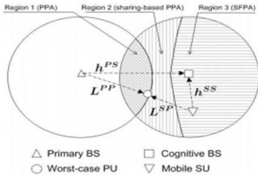
Figure 2.1: A CR framework existing together with an essential framework (uplink situation for the CR framework). Three locales are featured for the CR framework to work diverse power designation procedures
