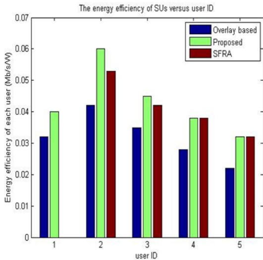
Figure 5: The energy efficiency of SUs versus user ID with different resource allocation strategies
