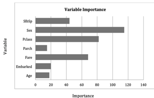
Fig. 2. Variable Importance for Titanic Dataset
