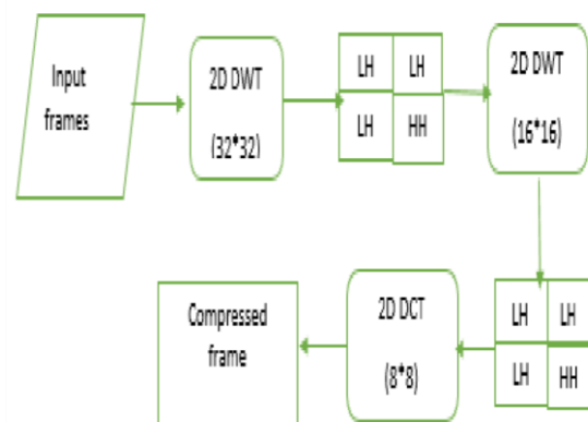
Fig 4:Flow chart of DCT-DWT block
