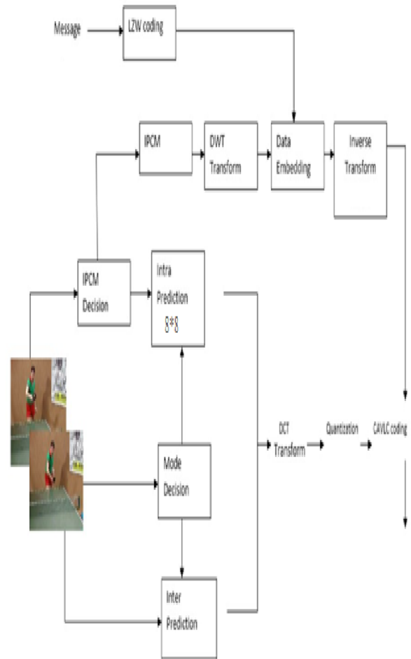
Fig 3:Detailed block diagram of proposed Data hiding in H.264/AVC
