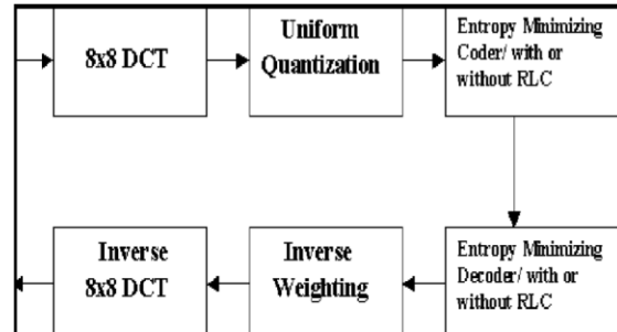
Fig 1: DCT block
