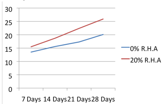
FIG: 1 Graph Shows Variation in Compression Strength
