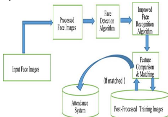
Figure-1 Basic representation of system architecture
