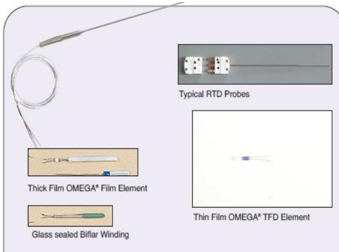
FIG- Typical RTD's
