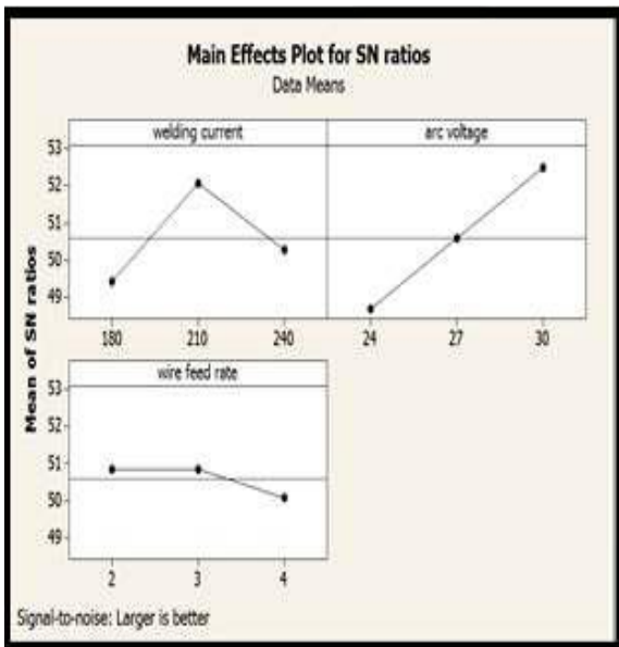
Fig.7 Main effect plot for SN ratios
