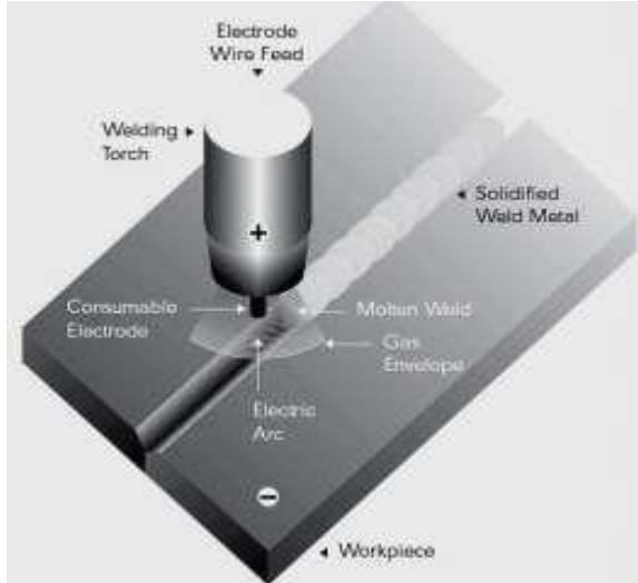
Fig.1 Basic working principle
