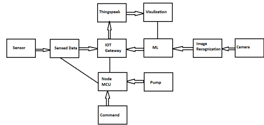
Fig-1: Prototype Of Smart Irrigation System using IoT
