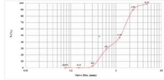
From graph: D_{10} = 0.40 , D_{30} = 0.65 , D_{60} = 1.80 C_u = 4.50 , C_c = 0.094
