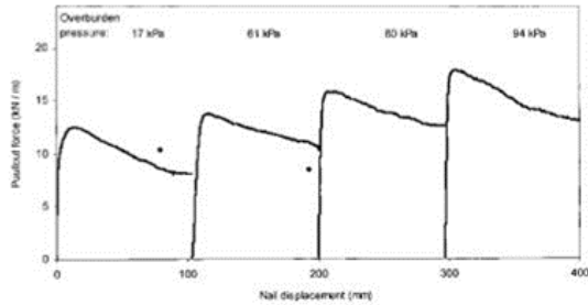
Fig. 5. Graph of force against displacement
