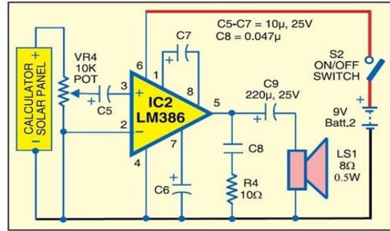
Fig. 4. LiFi Receiver circuit
