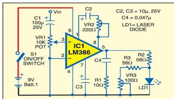
Fig. 3. LiFi Transmitter circuit
