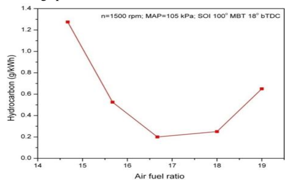
Fig.5. Hydrocarbon Vs air fuel ratio
