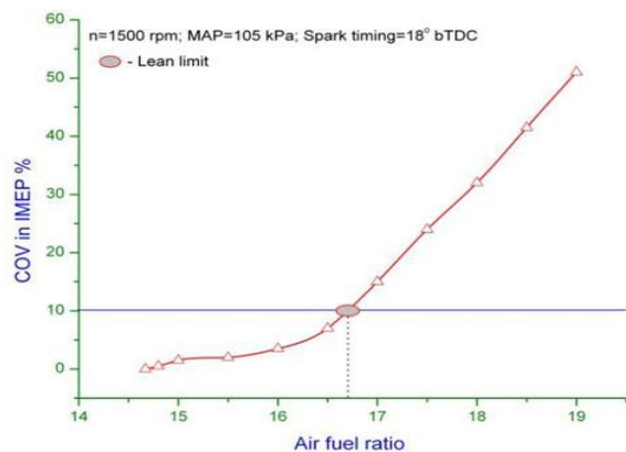
Fig.3. COV in IMEP Vs Air fuel ratio
