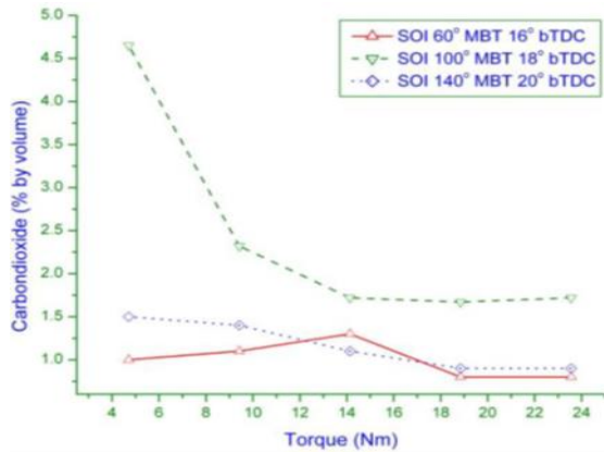
Fig.12. Carbon dioxide Vs Torque
