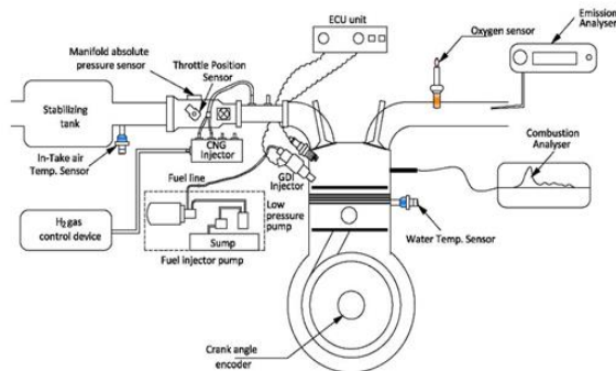
Fig.1. Experimental Configuration of GDI Engine
