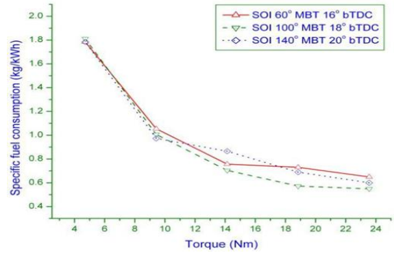
Fig.8. Specific fuel consumption Vs SOI
