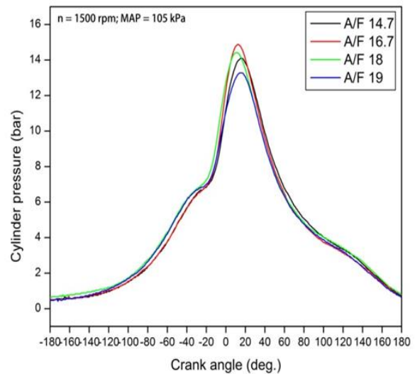
Fig.13. Cylinder pressure Vs crank angle
