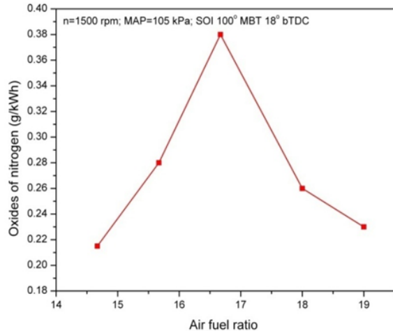
Fig.7. Oxides of nitrogen Vs air fuel ratio
