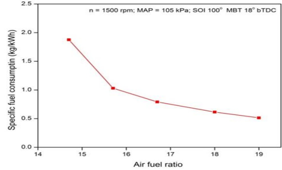
Fig.4. Specific fuel consumption Vs air fuel ratio
