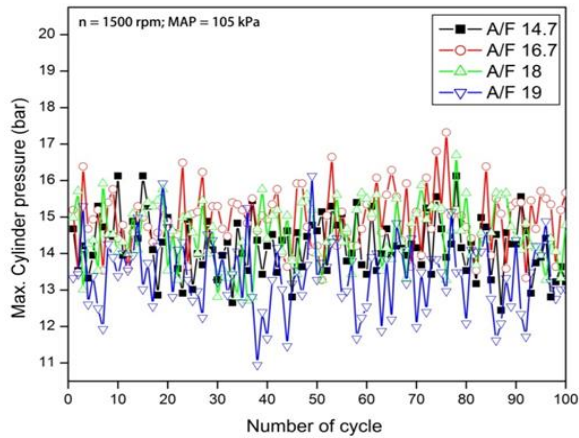
Fig.14. Maximum cylinder pressure Vs number of cycle
