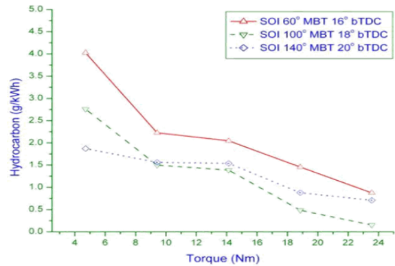
Fig.9. Hydrocarbon Vs Torque
