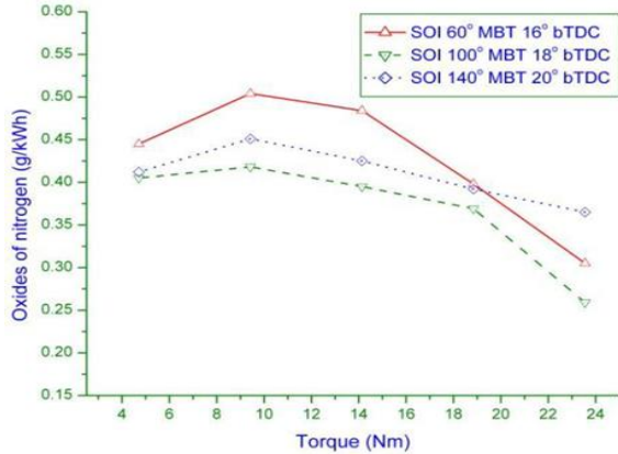
Fig.11. Oxides of nitrogen Vs Torque
