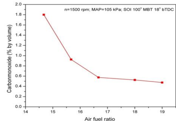
Fig.6. CO Vs air fuel ratio
