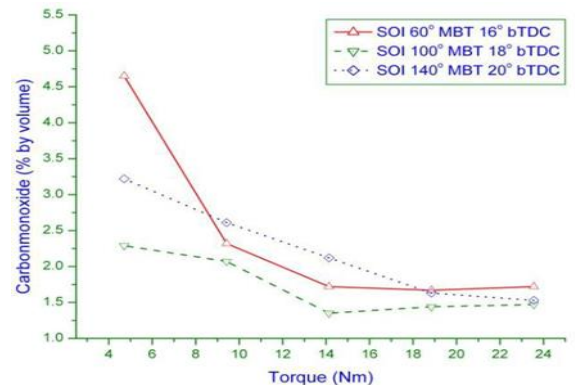
Fig.10. Carbon monoxide Vs Torque
