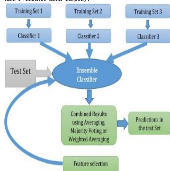
Figure 2- ML based Heart Diseases Prediction Model
