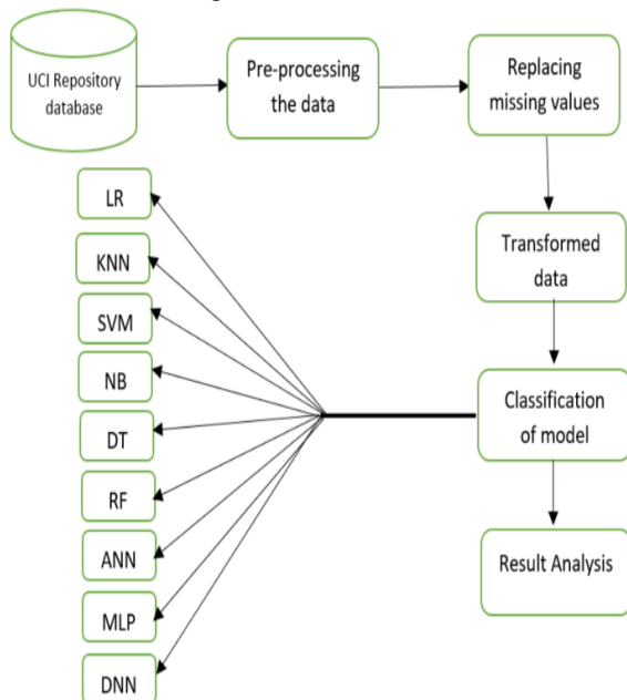
Figure 4- ML based Heart Diseases Prediction- A comparative study
