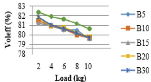
Fig-8: variation of volumetric efficiency with Load
