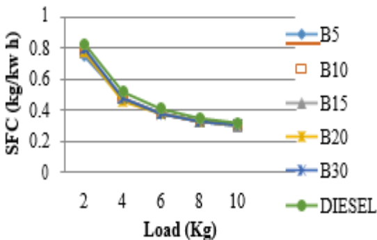
Fig-5: Variation of Specific fuel consumption with Load
