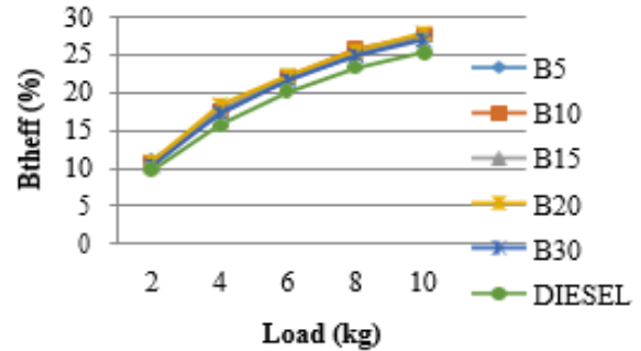
Fig-6: Variation of BTE with Load
