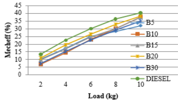
Fig-7: Variation of Mechanical efficiency with Load
