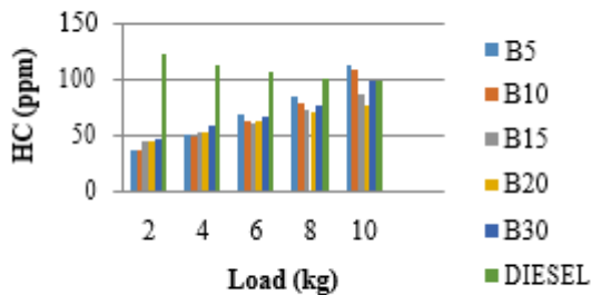
Fig-11: Variation of HC with Load
