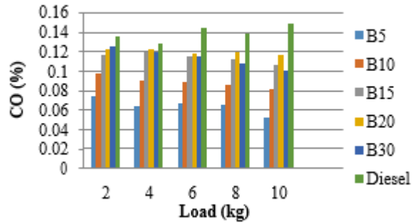
Fig-9: Carbon Monoxide with Load
