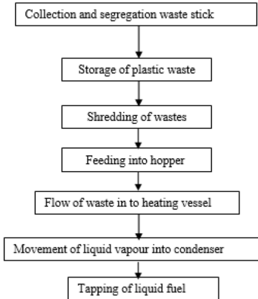
Fig -1: conversion of solid waste into liquid fuel
