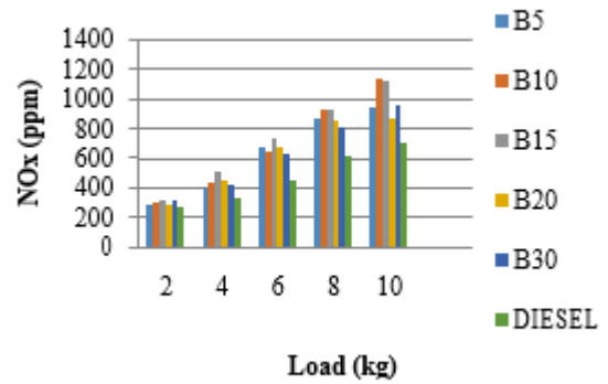
Fig-12: Variation of NO x with Load
