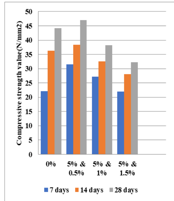
Fig 5.COMPARISON OF COMPRESSIVE STRENGTH TEST RESULTS
