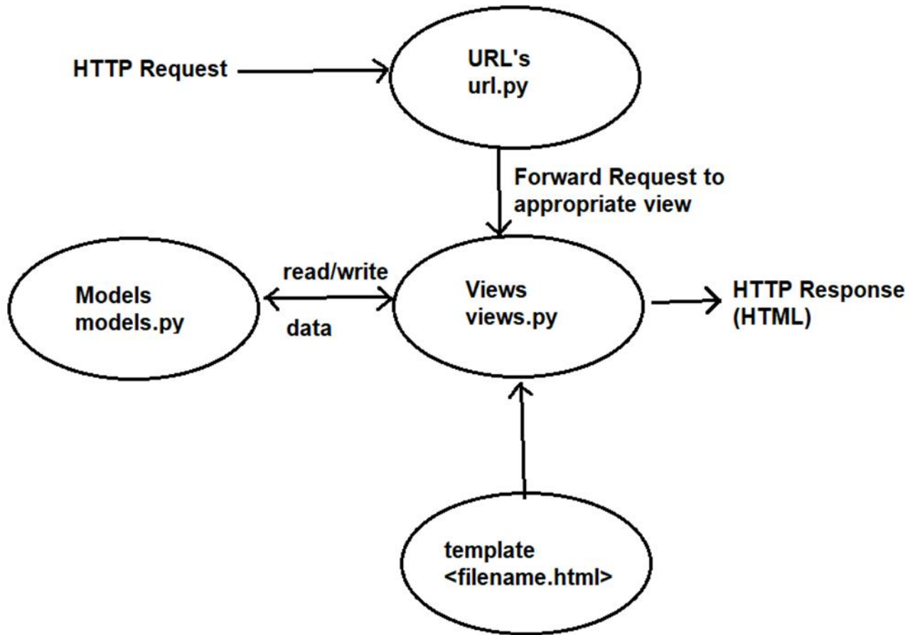
Fig 1.4: Model View Template of the System
