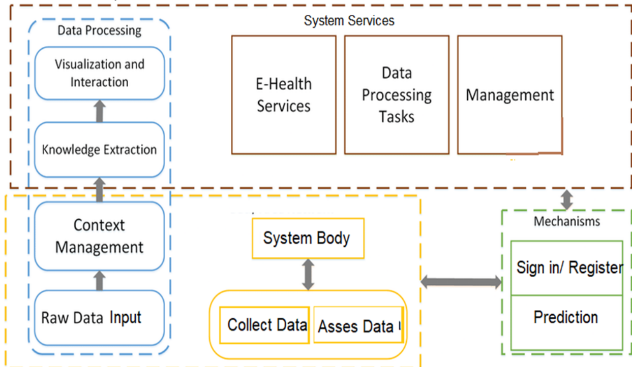
Fig 1.3: Architecture diagram of the system
