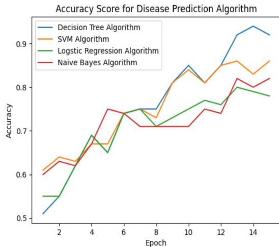
Fig 1.9: Depicts Accuracy Score at different epochs for different algorithms
