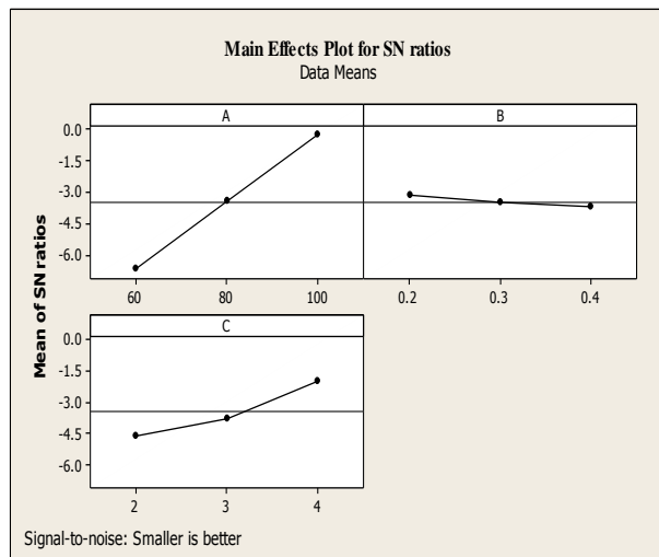
Fig. 3 Main effects plot for S/N ratio of SR.
