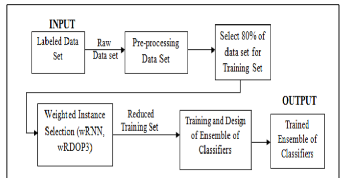
Figure 2: Architecture of the System
