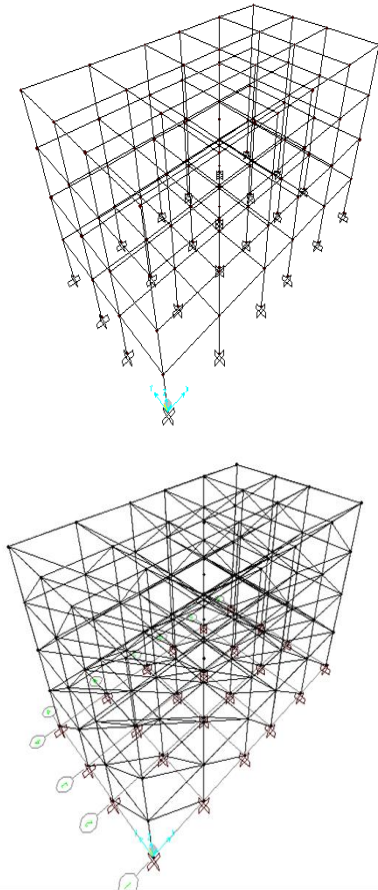
3D Computer model of building without and with considering infill stiffness respectively.(a) without infilla
