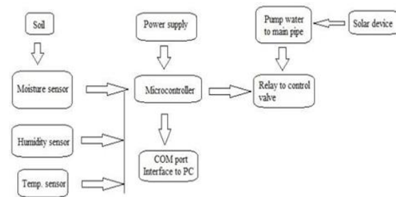
Fig.1. Block diagram of solar powered irrigation system
