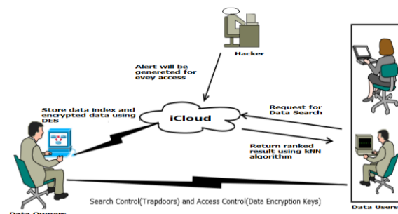
Fig1. System Architecture for search over encrypted cloud data
