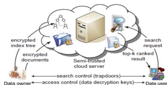
Fig.2 Architecture diagram of the MRSE Implementation.
