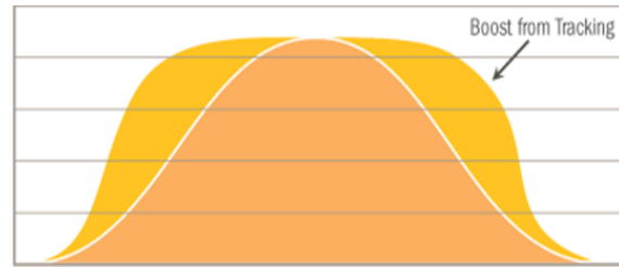
DAILY POWER PRODUCTION TRACKER COMPARED TO FIXED MOUNT FIG.3. AZIMUTH ANGLE ROTATION
