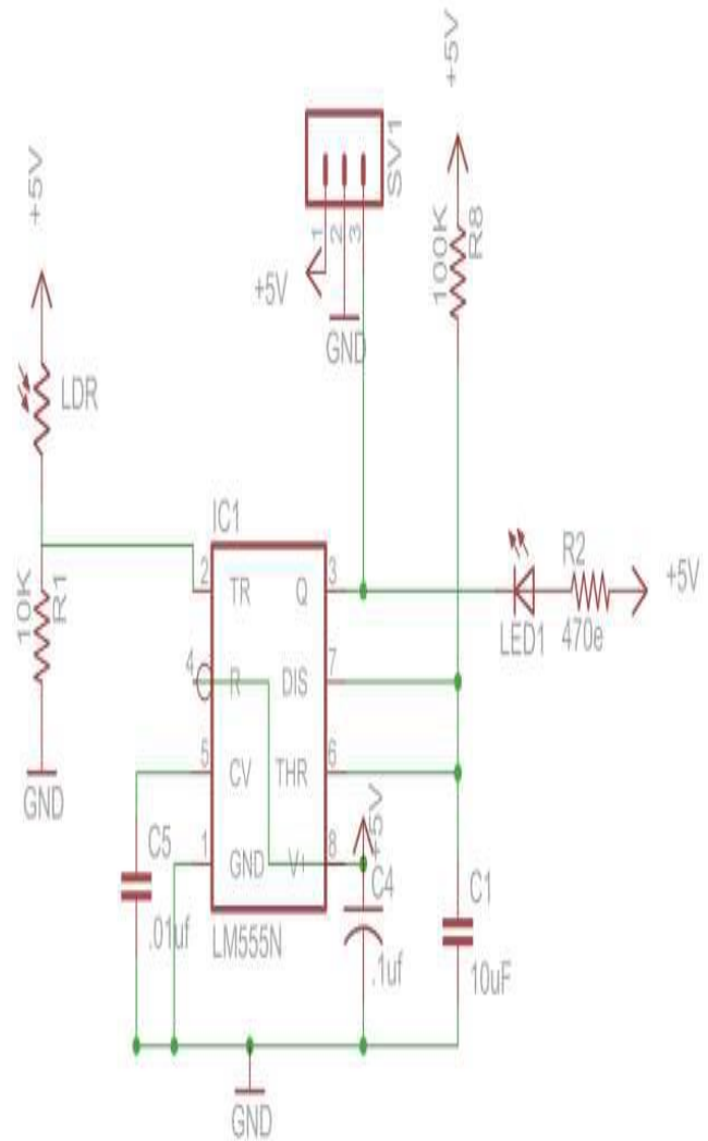
Fig.(ii) LDR Circuit
