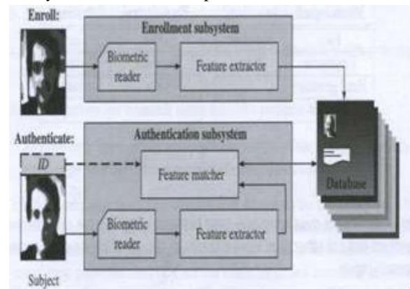
Fig 1: Typical Structure for Biometric Identification System
