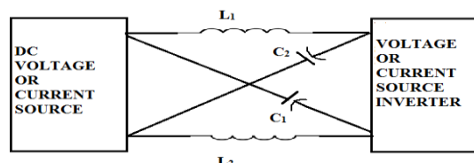
Fig.1. Z-Source Inverter
