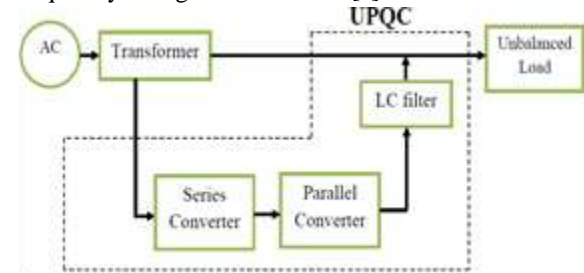
Fig. 1: Block diagram of UPQC
