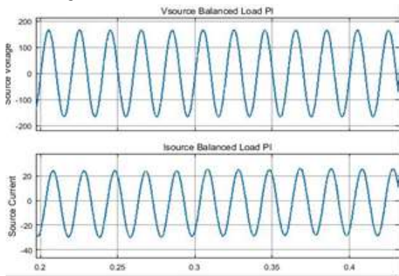
(a) Source voltage (b) Source Current
