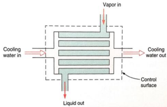
FIG:3 Layout of Water Cooled Condenser.
