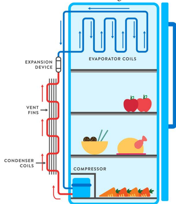
FIG: 1 Layout of Domestic refrigerator components.
