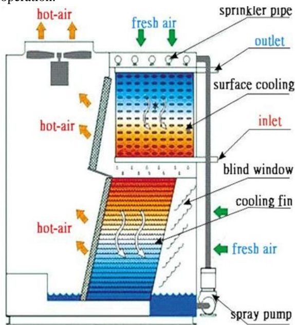
FIG:4 Layout of Evaporative Condenser.
