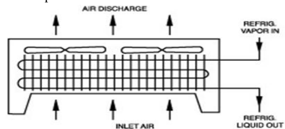
FIG:2 Layout of Air Cooled Condenser
