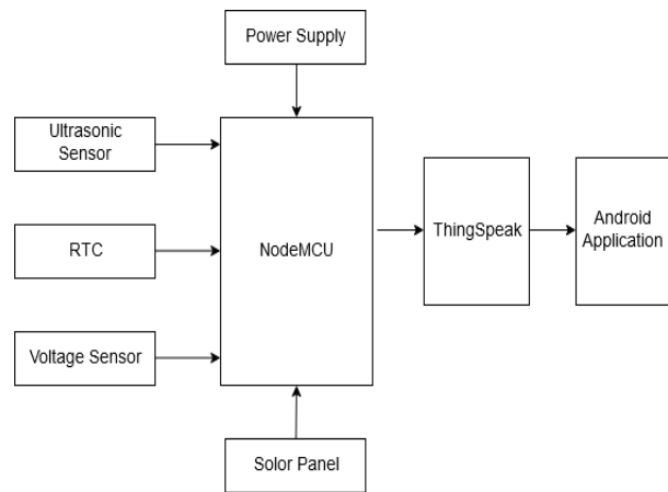
Fig 4.1 Architecture of smart dustbin
