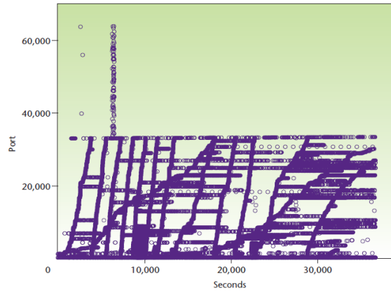
Figure 4. Port usage at MIT’s Lincoln Lab. This data set illustrates patterns in the use of source and destination ports over a 10-hour period. Dots indicate the use of a port at a particular moment in time.
