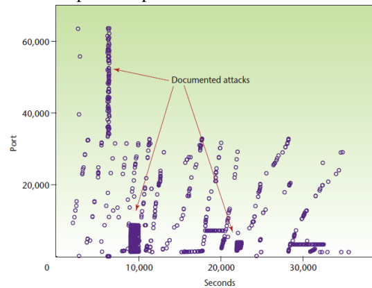
Figure 5. Anomalous port activity on the Lincoln Lab machines. Subtracting all (time,port) pairs that were active during the base comparison period in Figure 4 shows three areas that represent unusual port activity, which could be attacks.
