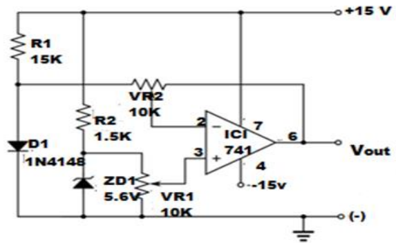
Fig-5 Circuit Diagram
