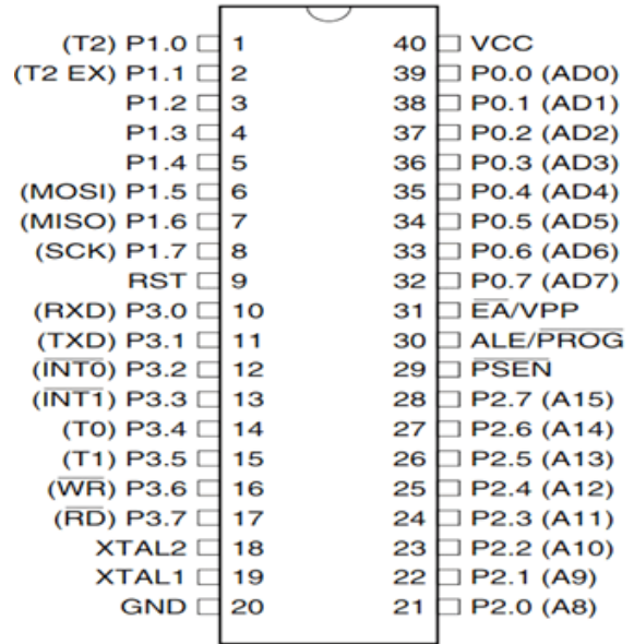
Fig:-1 Pin Diagram
