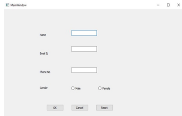
Figure 1 Registration page
