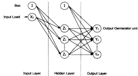
Fig. 3 Artificial neural networks structure for economic dispatch
