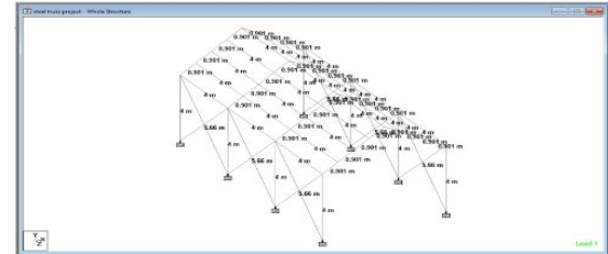
Figure1: 6m span hot rolled steel structure geometry with dimension
