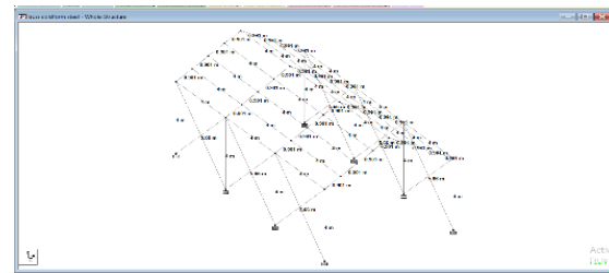
Figure2: 6m span cold formed steel structure geometry with dimension
